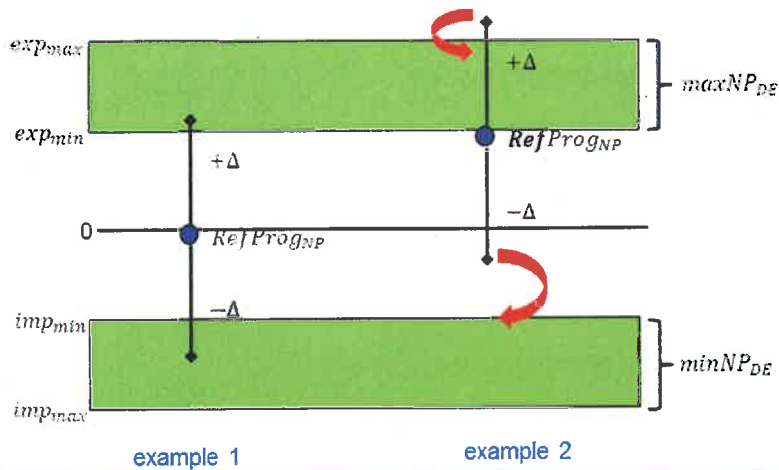
Figure 4-3: Export/import limits illustration.
