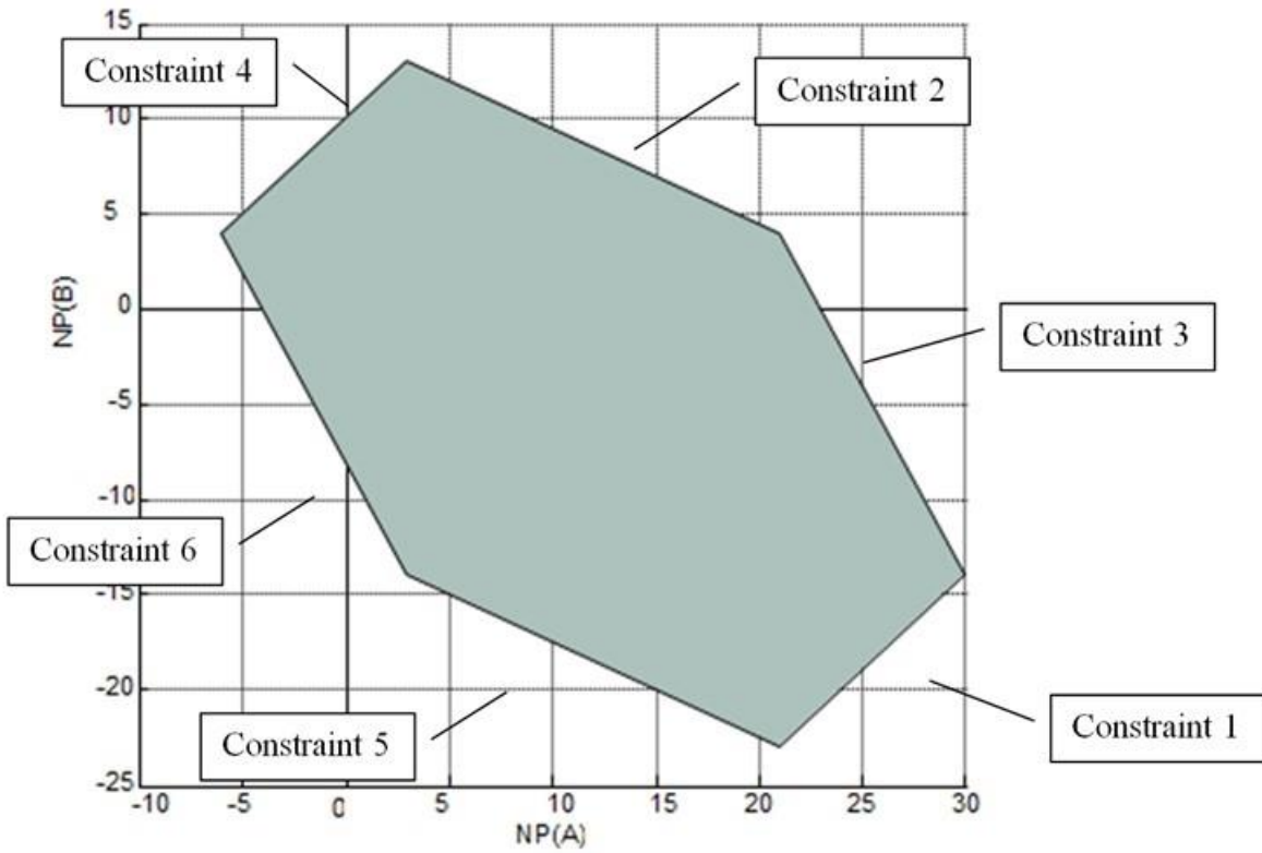
Figure 25: FB domain
